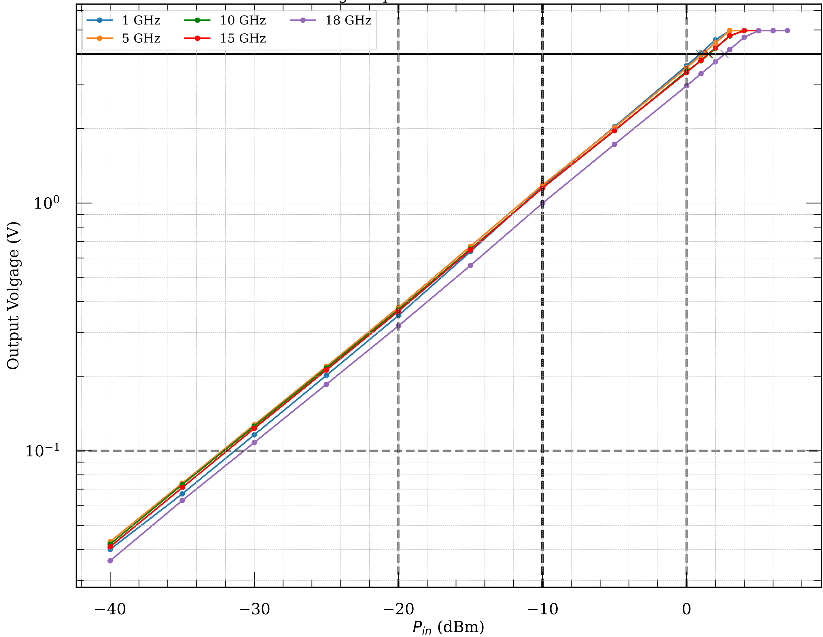
Measured voltage-to-power curve of detector module004v2
